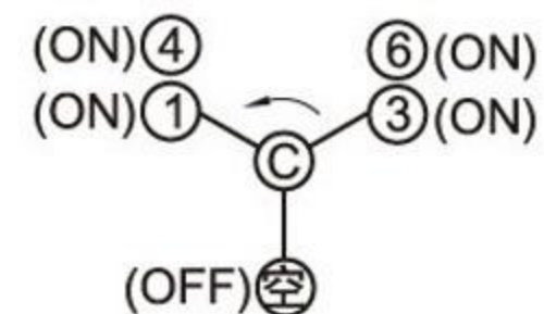
ON-ON-OFF SCHEMATIC (NON-SHORTING)
